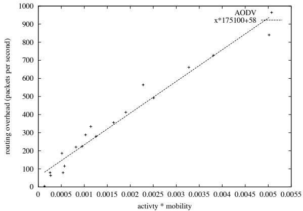
(b) AODV
