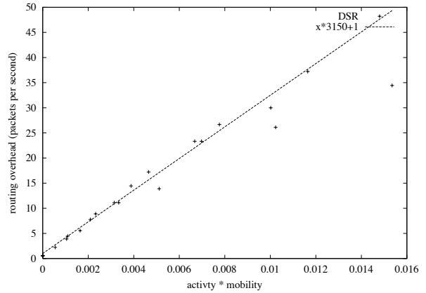
(a) DSR
