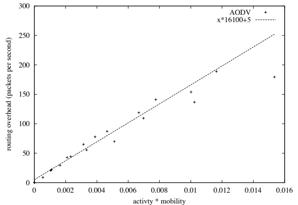
(b) AODV
