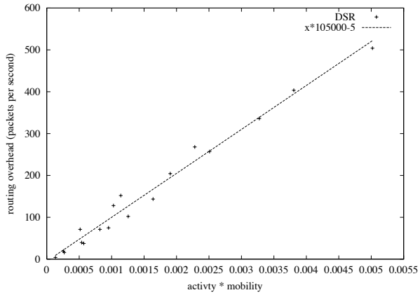
(a) DSR
