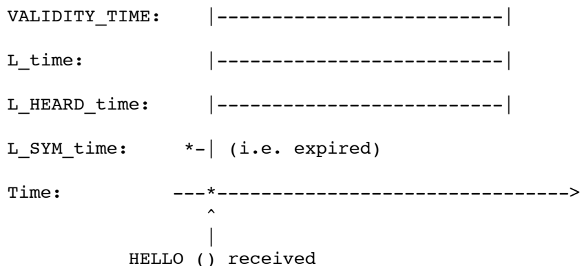
Figure 6: HELLO message processing: network address not present
