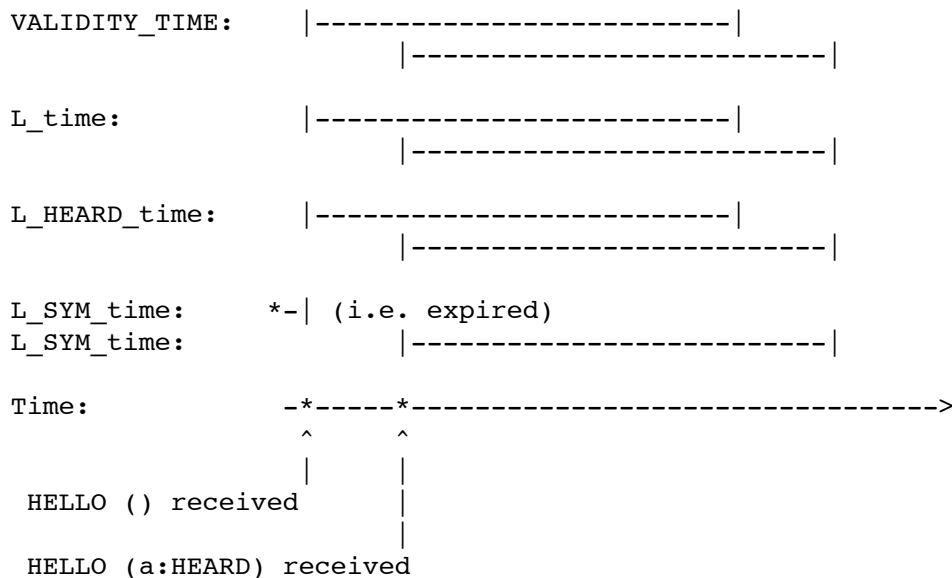
Figure 7: HELLO message processing: network address present
