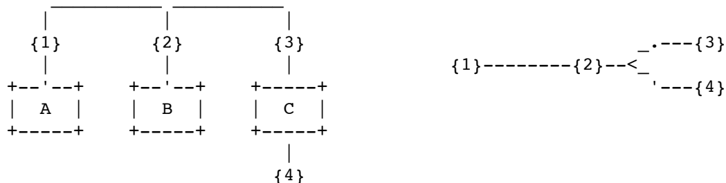
Figure 16: Single addresses, with 2-hop neighbor C having two interfaces (left), and corresponding NHDP representation (right)
