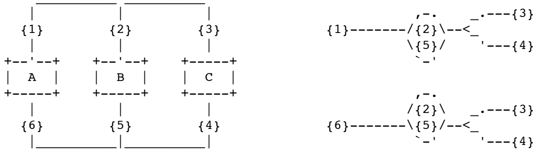
Figure 20: Single addresses, with all routers having two interfaces (left), and corresponding NHDP representation (right)
