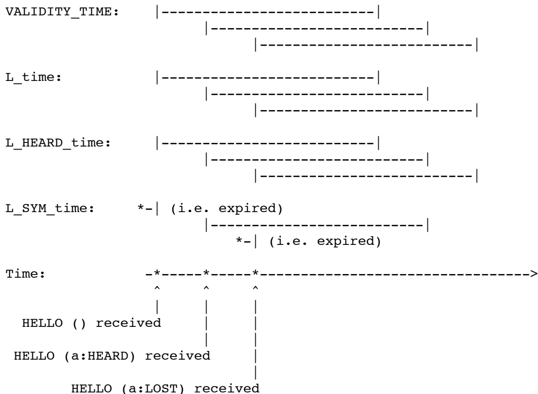
Figure 8: HELLO message processing: network address lost
